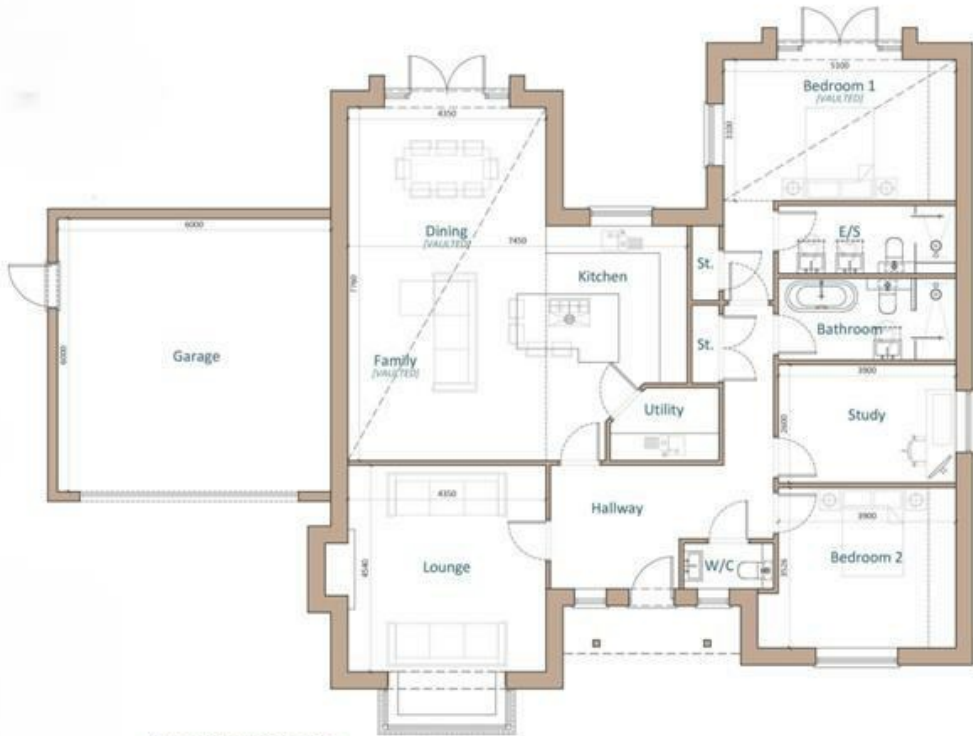
Proposed Ground Floor Plan Scale 1:50
